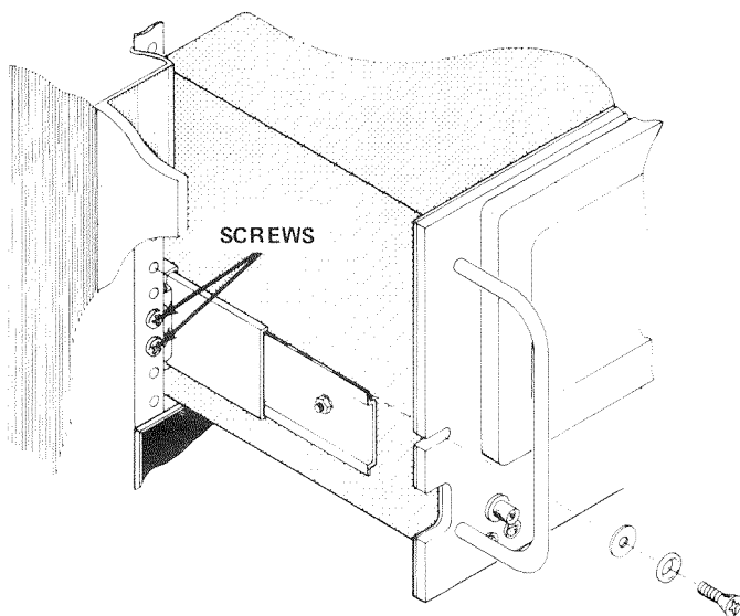
Figure 3-5. Adjusting the slide out tracks for smooth sliding action.
